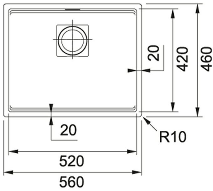
Technical Drawing
